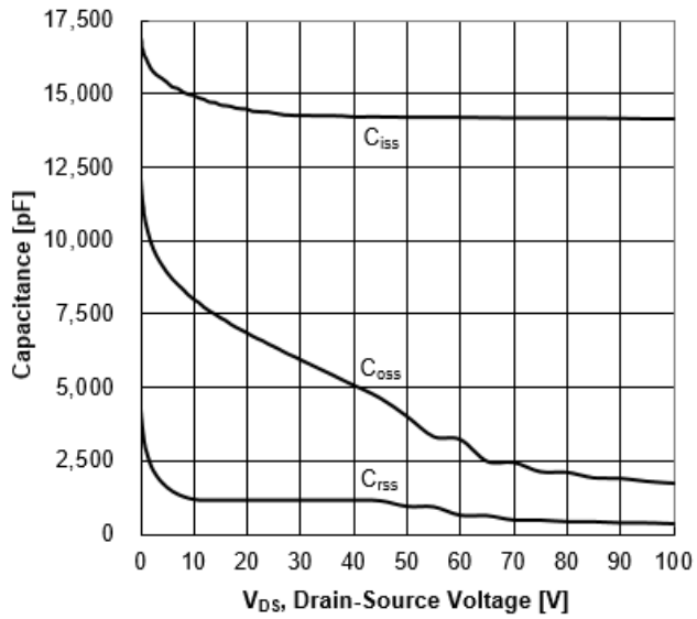
Figure 12. Capacitance Characteristics
